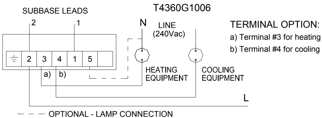
Fig 4: T4360G1006 (Heat or Cool, light operates on temp fall) wiring diagram
