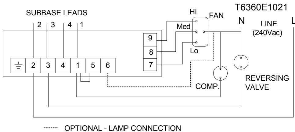
Fig 8: T6360E1021 (Heat Pump Heat/Off/Cool Lo/Med/Hi Fan) wiring diagram
