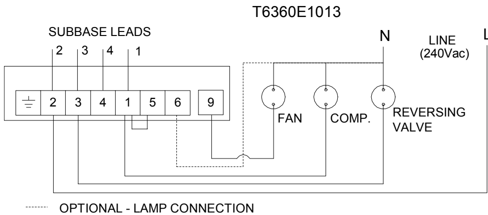
Fig 7: T6360E1013 (Heat Pump Heat/Off/Cool Cont/Auto Fan) wiring diagram
