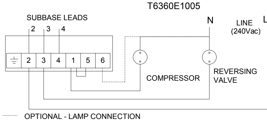
Fig 6: T6360E1005 (Heat Pump Heat/Off/Cool) wiring diagram
