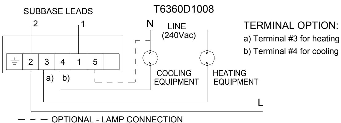
Fig 5: T6360D1008 (Cool or Heat, light operates on temp rise) wiring diagram
